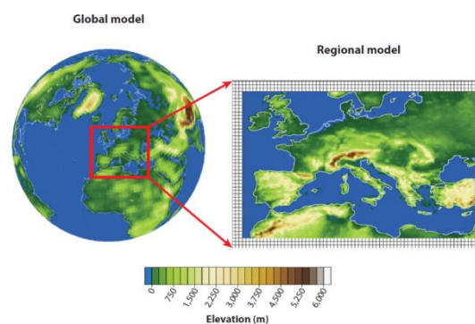
Figure 5 - Schematic depiction of the dynamical downscaling technique.
